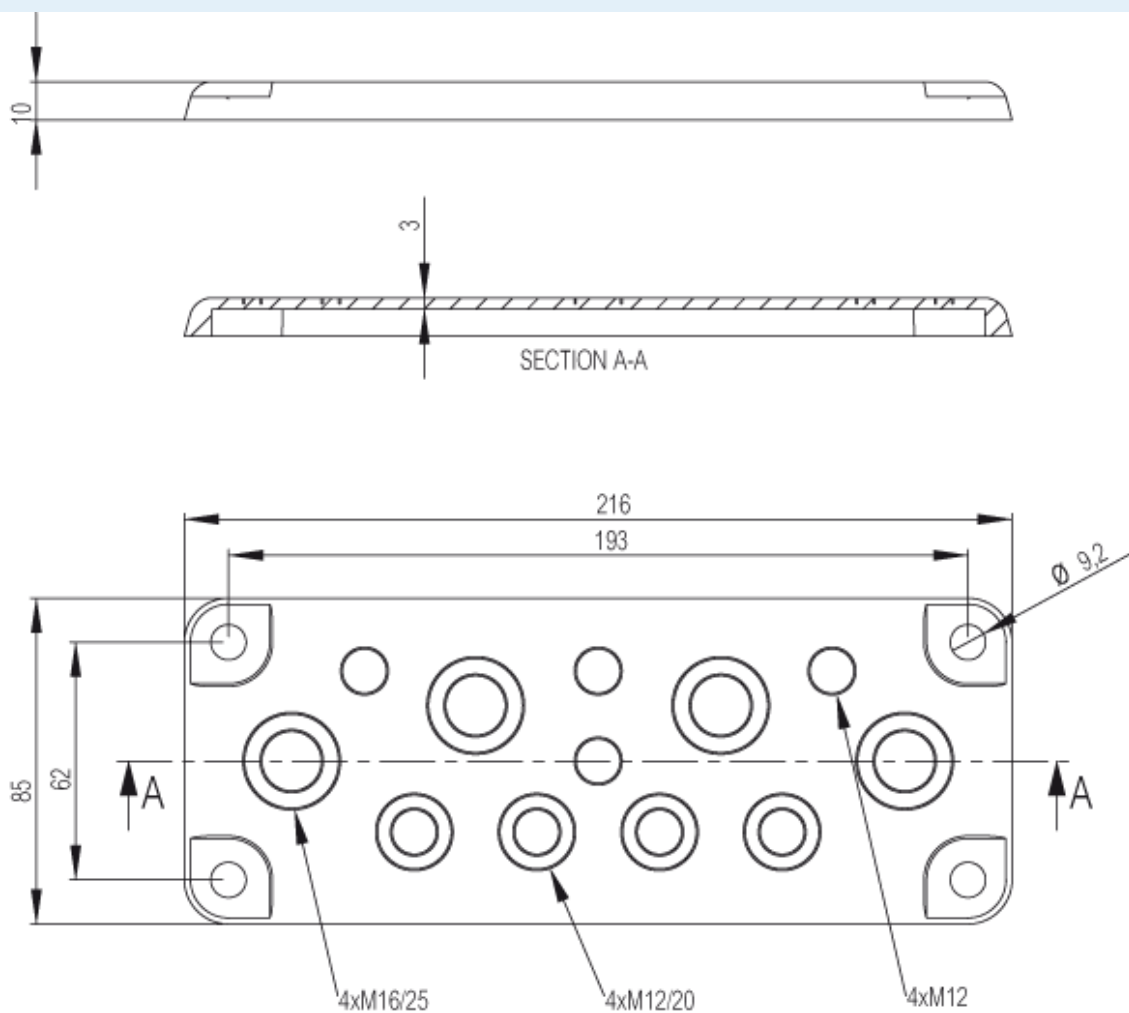
FIBOX MB 10857
