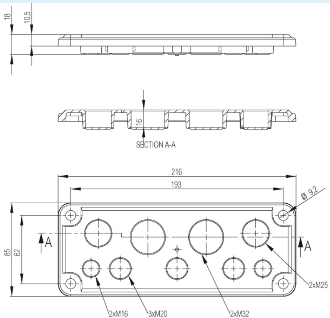
FIBOX MB 10862
