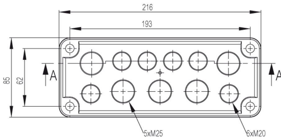
FIBOX MB 10860
