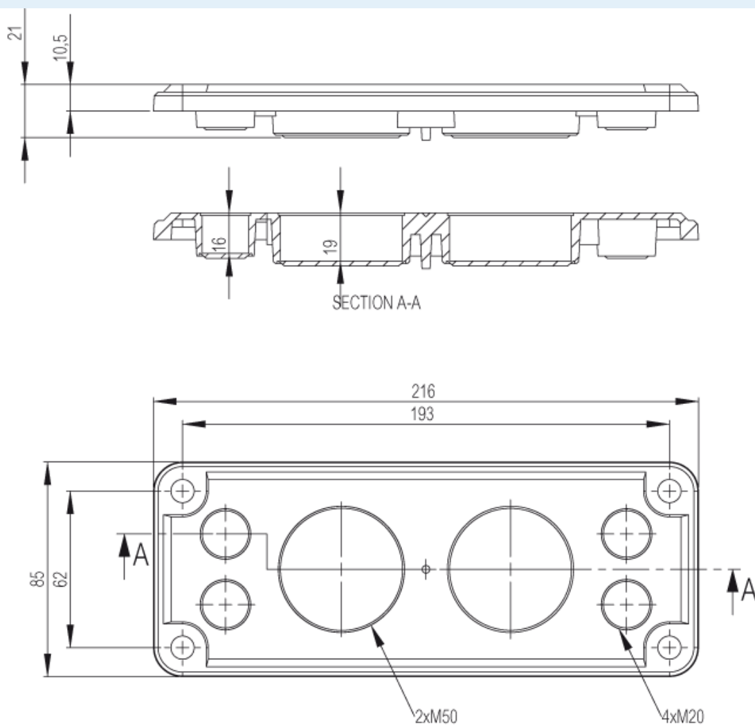
FIBOX MB 10861
